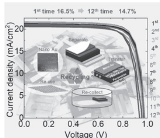
Fig. 3 Schematic of recycle utilization of nano-porous Au electrode for perovskite solar cell, and its photovoltaic performance in recycled utilization of electrode.
