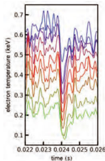
Bursty transport observed in torus plasmas. Heat is transferred to outside of plasma. This phenomenon is similar to avalanches, which are driven by self-organized criticality of turbulent plasma.
