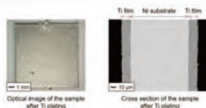
Obtained Ti films with smooth surface by the molten salt electroplating
