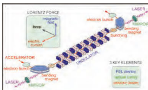
Principle of FEL
