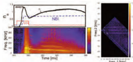
Measurement and signal processing for the turbulent plasma fluctuations. Various spectral analysis techniques are useful for determining the eddy size, frequency and non-linear coupling of the turbulences.
