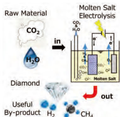
Production of useful substances from carbon dioxide by molten salt electrolysis.
