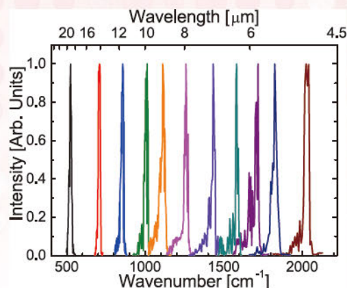
Wavelength Tunability of KU-FEL
