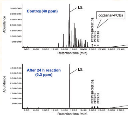
D. The result of reacting 40 mg L -1 of commercial PCBs with composite type of catalytic enzyme, it degraded to 0.3 mg L -1 in comparison with the control (top) within 24 hours (bottom). PCBs was analyzed by gas chromatograph quadrupole mass spectrometer.
