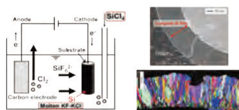
A new production method of silicon films for solar cells by the molten salt electroplating
