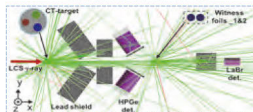
Isotope CT by using Laser-Compton Gamma-ray beam
